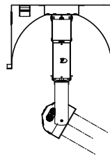
One-Lamp Drop-Pan-Tilt (shown in dropped position and tilted)
