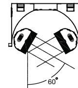
One-One-Lamp Rotate with maximum left and right slide; includes contrast feature
