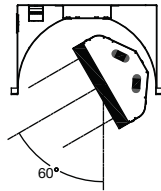
Two-Lamp Rotate with maximum right slide; includes contrast feature
