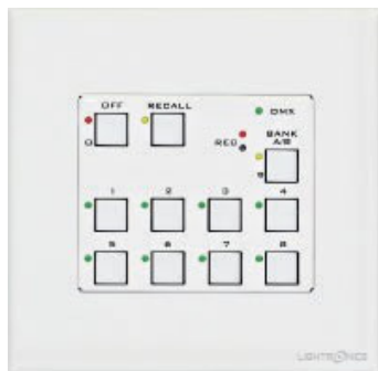
Wall Mounted Playback Station (P/N CTRL-WS-LV-SR517)
